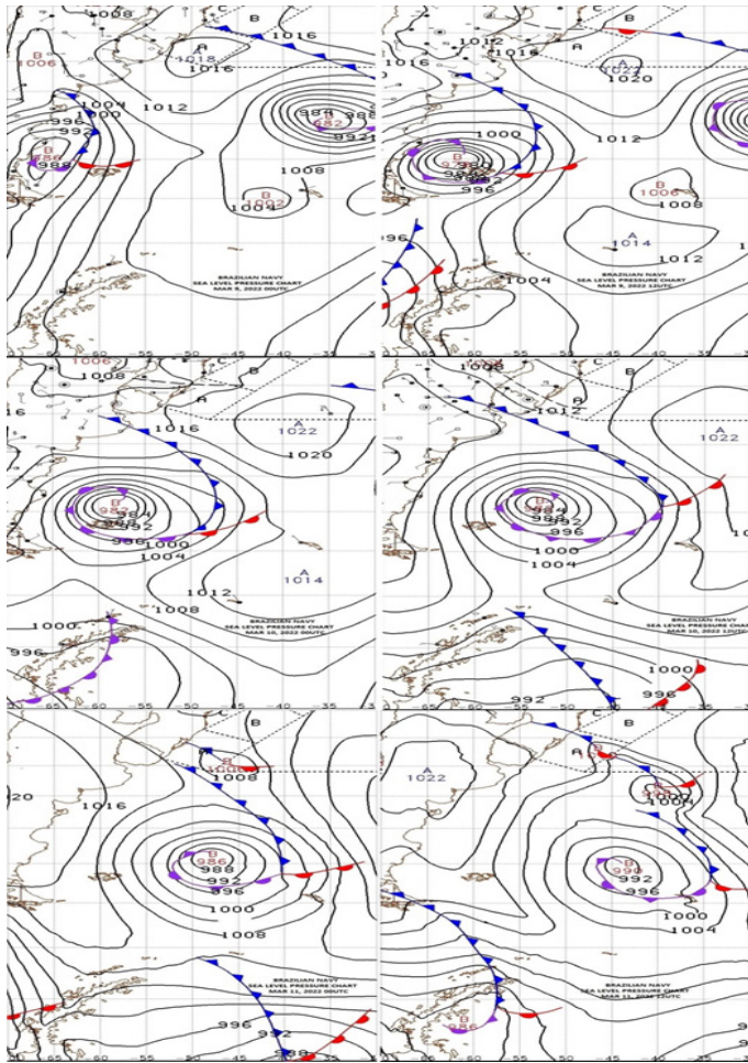
Figure 8. The Synoptic Letters, from March 9, 2022, at 00:00 UTC to March 11, 2022, at 12:00 UTC, from Navy Hydro-raphy Center, Brazil's navy.
