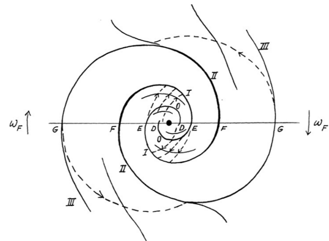
Figure 9. The application to the permanence of the spiral structure in galaxies arises because the outermost part of an arm will be attracted by, and will tend to become assimilated with, the neighboring parts of the inner structure. In an analogous way matter close to the nucleus will have a tendency to be assimilated in an outward motion with the inner parts of the spiral structure. The two regions of circulation are given here. We may suppose that there are two points F in the structure where the angular motion \omega_F is equal to the local circular angular velocity. We can introduce a coordinate system which follows \omega_F center. The successive inter-sections with the diameter through the points F are indicated by the letters D, E, F, and G. We make the supposition that, as long as the mass of III is small, the motion of particles in the arcs II is circular motion in the general gravitational field. The gravitational force from the interior spiral structure will not appreciably change the radial direction of the general field, of which it will form an integral part.", (Lindblad, 1964) [24].
