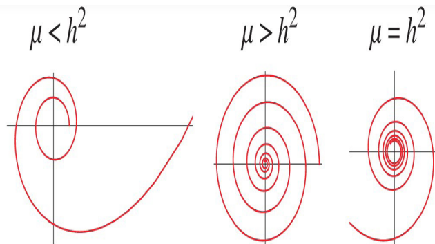
Figure 7. Represents the three possible shapes of the Cote's Spiral.
