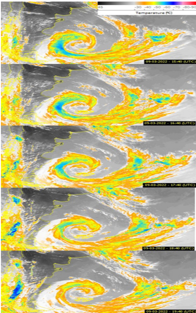
Figure 2. Enhanced satellite images (Adapted) taken from the REDEMET website for cloud temperature data between March 09, 2022 15:40 UTC to 19:40 UTC.
