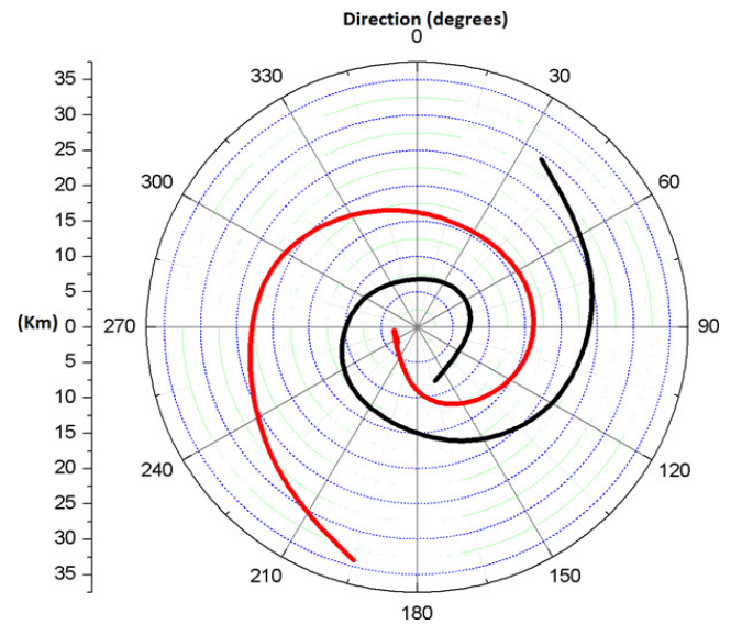
Figure 10. Graph built with the data collected from Figures 5 and Figure 6. The graphic depicts two spirals, constructed with the coordinates of the atmospheric pressure gradients by the wind speed tangent in the vortex of the extra tropical cyclone that passed north of the Falklands Islands.
