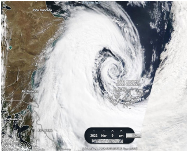
Figure 5. Satellite image of Powerful extra tropical cyclone over the Falkland Islands in this Wednesday, March 9, 2022 am. Source [28].
