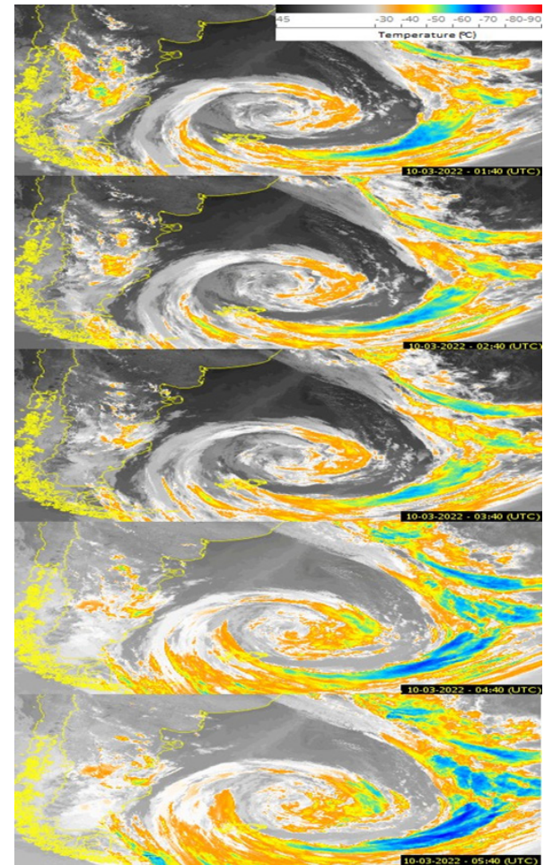
Figure 4. Enhanced satellite images (Adapted) taken from the REDEMET website for cloud temperature data between March 10, 2022 01:40 UTC to March 10, 2022 05:40 UTC.
