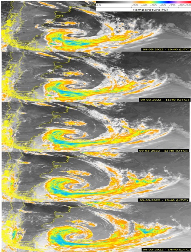
Figure 1. Enhanced satellite images (Adapted) taken from the REDEMET website for cloud temperature data between March 09, 2022 10:40 UTC to 14:40 UTC.
