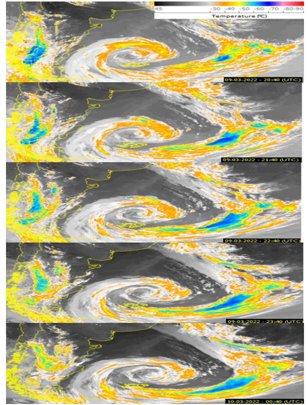
Figure 3. Enhanced satellite images (Adapted) taken from the REDEMET website for cloud temperature data between March 09, 2022 20:40 UTC to March 10, 2022 00:40 UTC.
